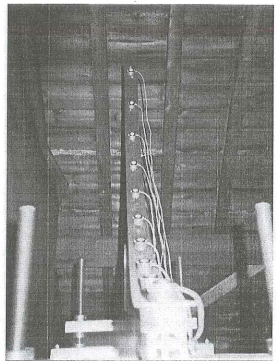
Figure 1 Apparatus to measure luminous intensity distribution from pipe emitter
