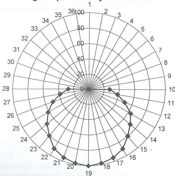
Figure 4 Polar curve of average luminous intensity distribution from overcast sky
